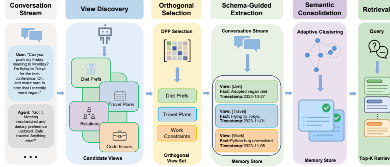
Fig. 1. The AutoViewMem architecture. The system processes a conversation stream through online view discovery, selects an orthogonal view set via DPP, and performs schema-guided memory extraction and retrieval to provide context for the LLM agent.
